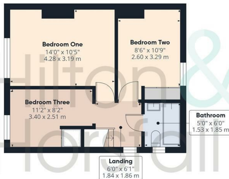
Floor 1 Building 1
